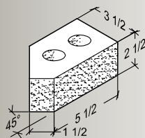
45° Squint
