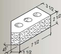
45° Squint
