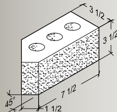
45° Squint
