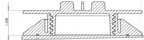
SECTION E-E
