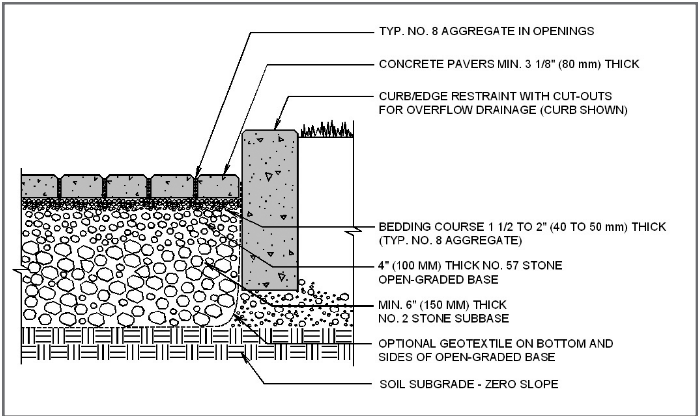
Typical installation for exfiltration.
