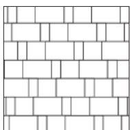
Mod. Running Bond 17% Single 33% Double 50% Triple
