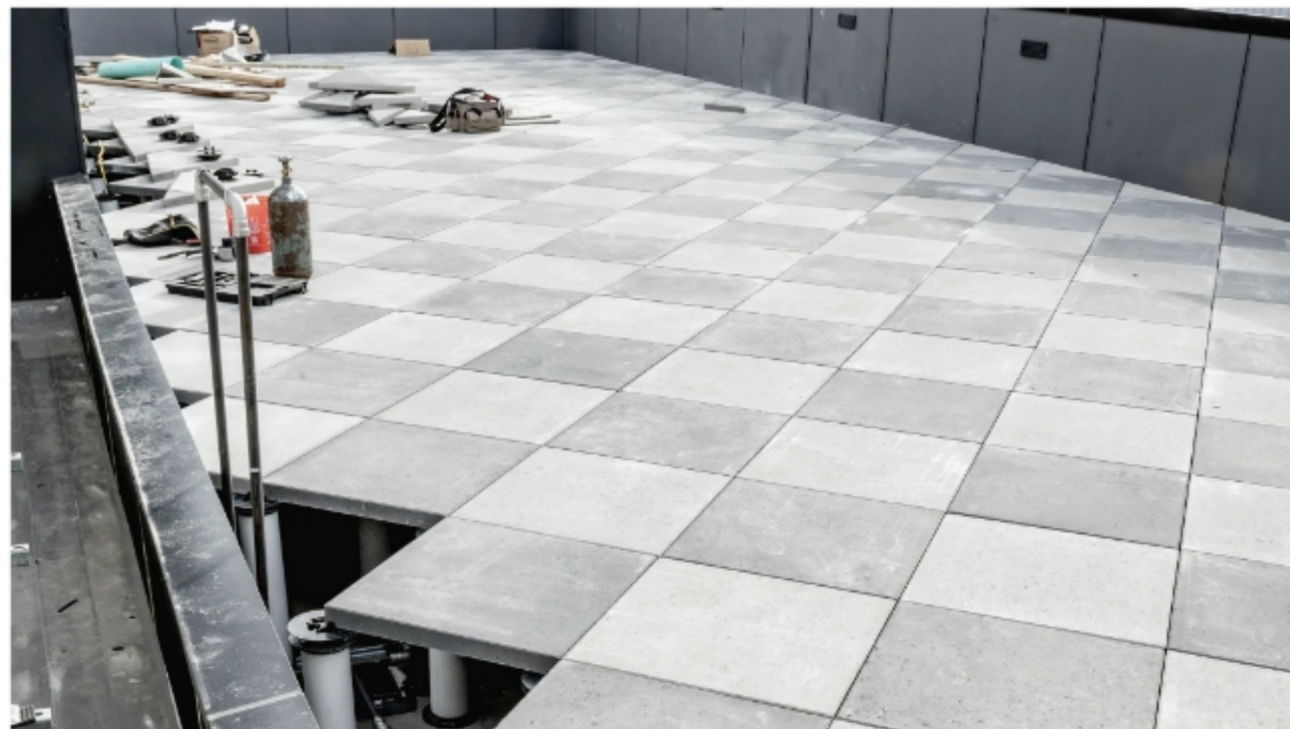
PICTURED: Pedestal Set Vancouver Bay Architectural Slab In Charcoal and Grey, Stacked Bond (Squares) Layout
